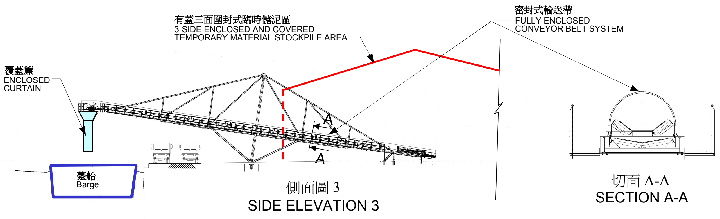
臨時躉船轉運站側面圖 SIDE ELEVATIONS OF THE TEMPORARY BARGING POINT
