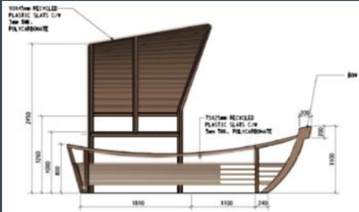
Sampan Seating Elevation 舢舨立面圖
