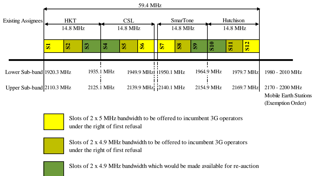
Figure 2 – Proposed Band Plan for Re-assignment of the Frequency Spectrum in the 1.9 - 2.2 GHz Band
