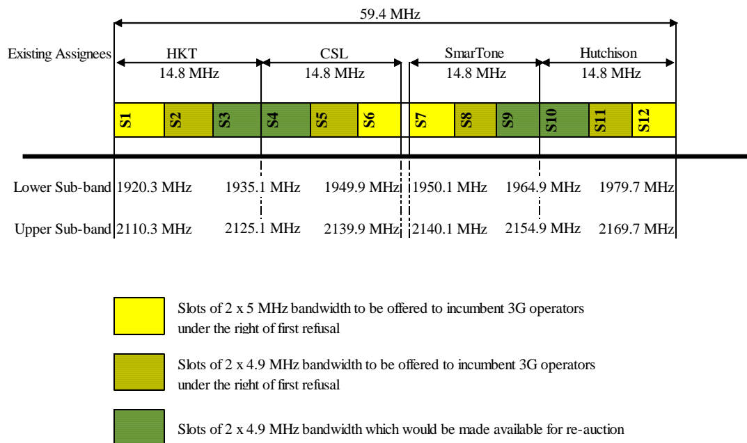
Figure 1: Band Plan for Re-assignment of the Frequency Spectrum in the 1.9 – 2.2 GHz Band
