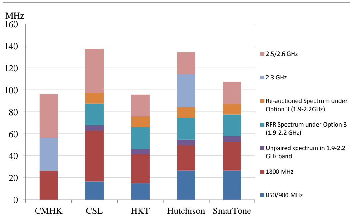
Figure 1: Distribution of Spectrum among MNOs for the Provision of Public Mobile Services
