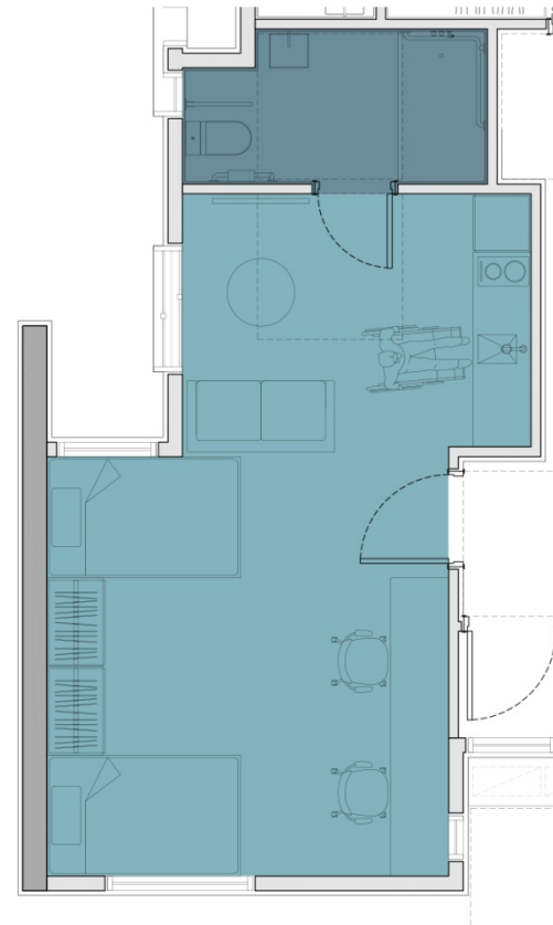
十九樓特別需要人士單位 19th Floor Special Needs Unit Plan
