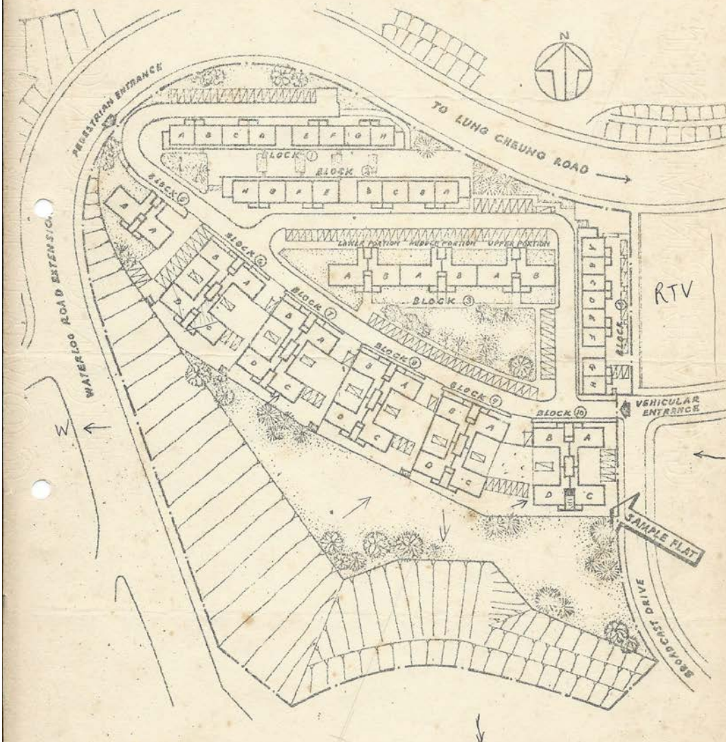
LAYOUT PLAN
