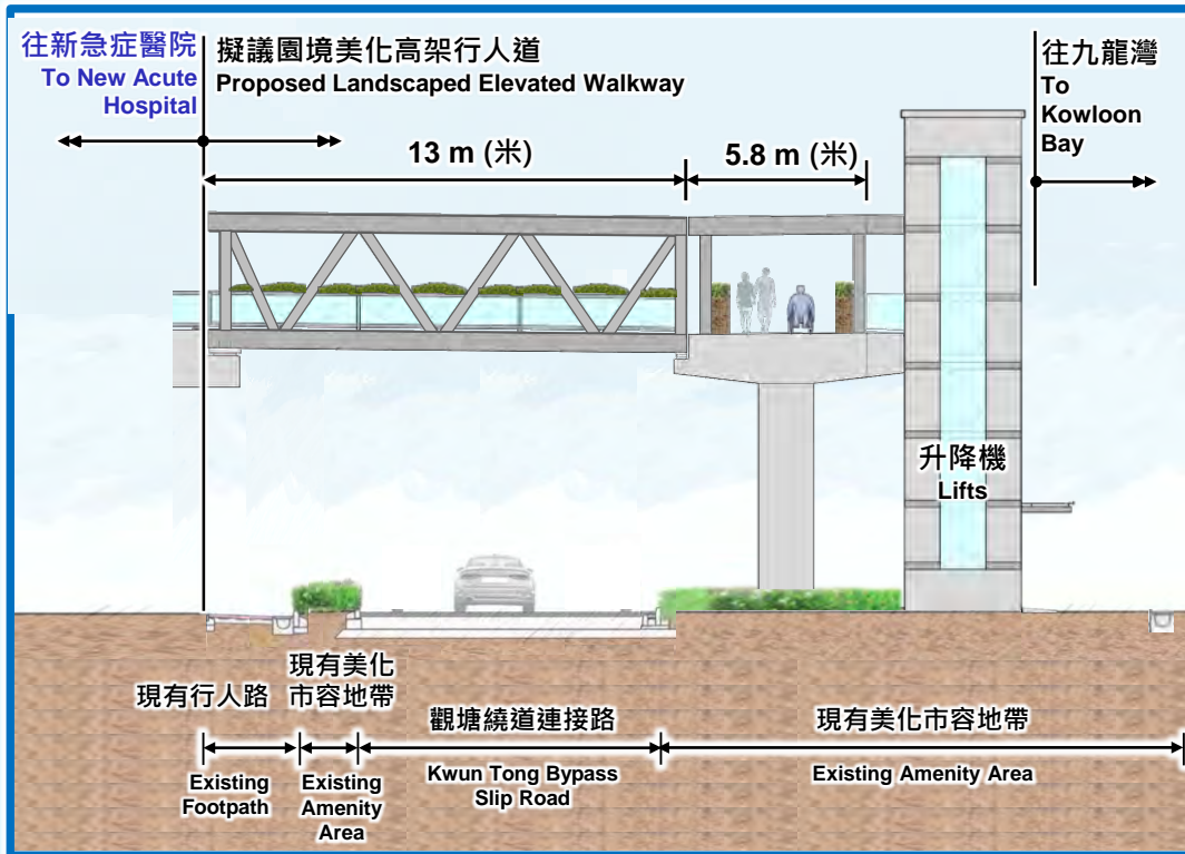
擬議園境美化高架行人道 (構想圖) 橫切圖 A - A Proposed Landscaped Elevated Walkway (Artist Impression) Section A - A
