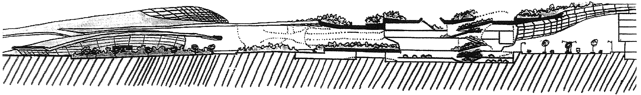
SECTION B-B (SCALE 1:1000)
