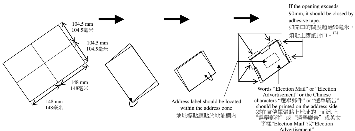
Figure 3 : Folder of A4 (296mm) size with 2 folds
