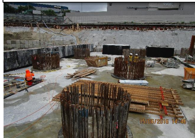
Formwork Erection for Large Pile Cap 大型樁帽模板搭建工程
