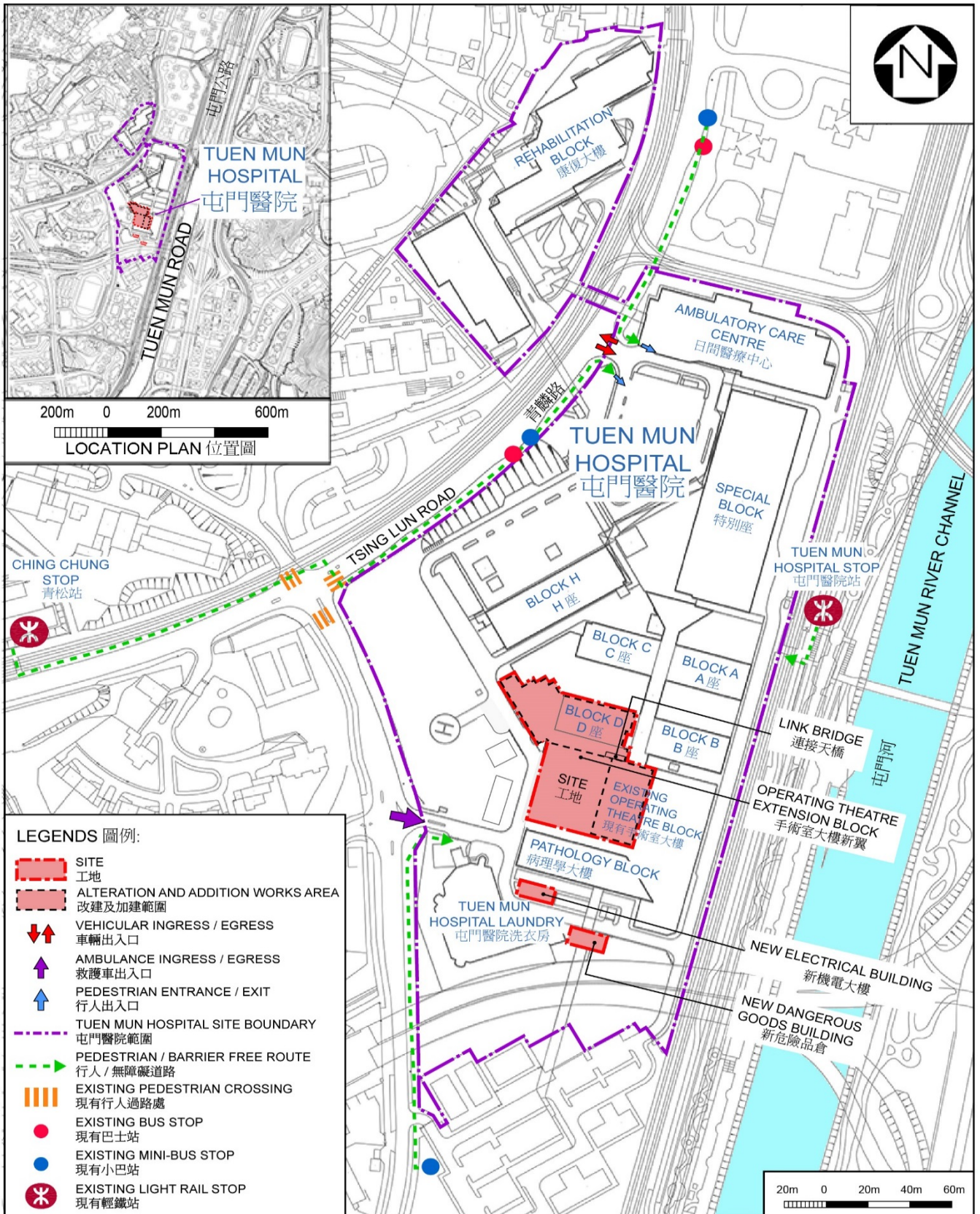
SITE PLAN 工地平面圖 86MM EXTENSION OF OPERATING THEATRE BLOCK FOR TUEN MUN HOSPITAL 屯門醫院手術室大樓擴建計劃
