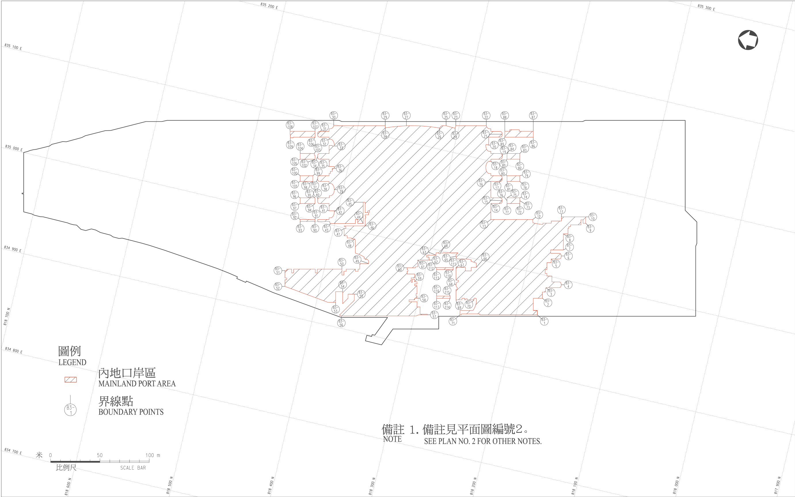
平面圖編號3：廣深港高速鐵路香港段 西九龍站B3層 - 內地口岸區界線點 PLAN NO. 3 : HONG KONG SECTION OF GUANGZHOU-SHENZHEN-HONG KONG EXPRESS RAIL LINK B3 LEVEL OF WEST KOWLOON STATION - BOUNDARY POINTS OF MAINLAND PORT AREA
