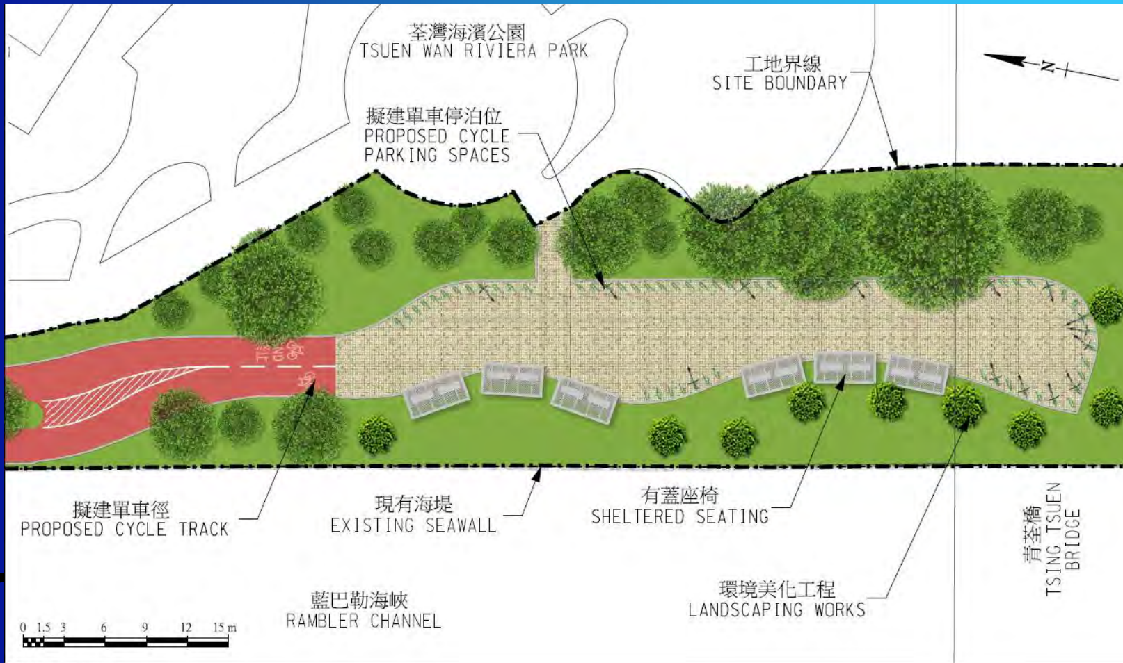
青荃橋附近休息處 平面圖 LAYOUT OF THE RESTING STATION NEAR TSING TSUEN BRIDGE
