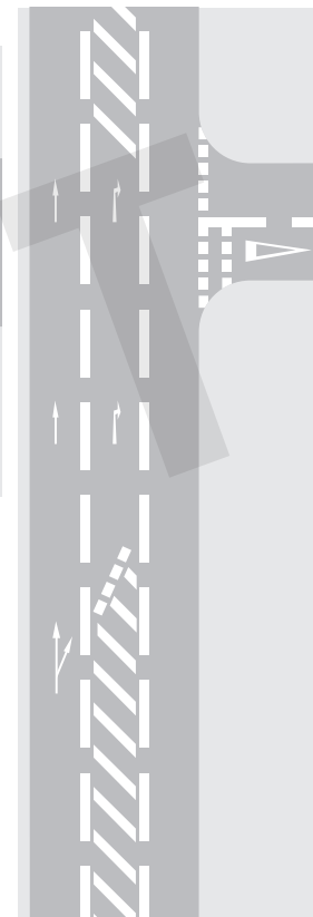
A right-turn lane formed with hatched markings to protect the right-turn traffic
