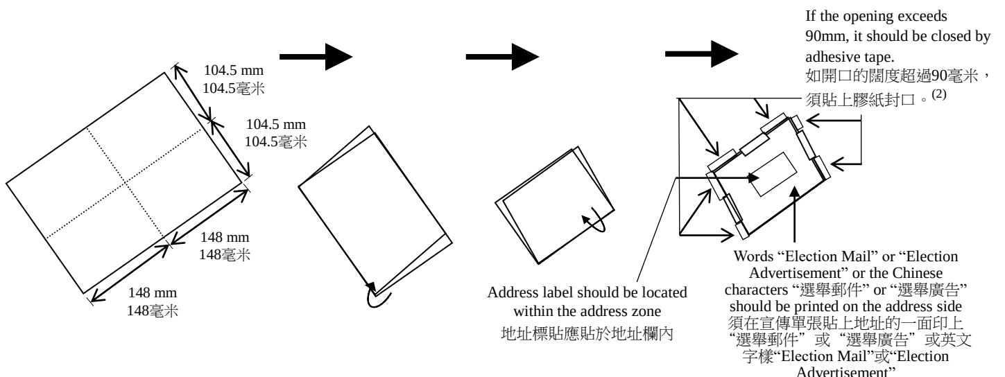
Figure 3 : Folder of A4 (296mm) size with 2 folds
